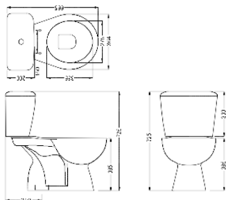
115070030S Acolia Ambra 843 Washdown Close Coupled WC S Trap: 250mm Size: 665 x 360 x 725 (mm)
