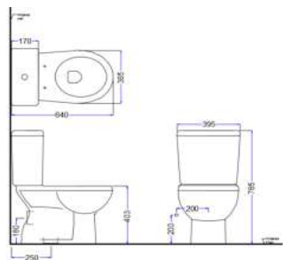
115010120 ACL 640PS Washdown Close Coupled WC S Trap: 250mm Size: 640 x 395 x 785 (mm)
