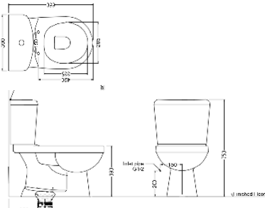
115070019SS ACL Ambra 842 Washdown Close Coupled WC S Trap: 250mm Size: 650 X 390 X 740 (mm)
