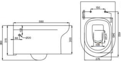
115010280 Acolia Bellino 5520W Wall Hung Toilet (P Trap) Size: 550 x 360 x 405 (mm)
